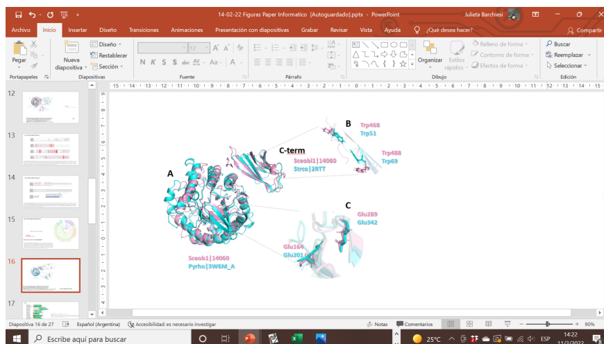
Fig. 7 3D modeling of GH5 endoglucanase 14060 from Scenedesmus obliquus UTEX B 3031. A. Proposed model of Sceobl1|14060 (pink) superimposed to Pyrhol3W6M_A GH5 and Strco|2RTT_A CBM2 templates (cyan); putative catalytic and binding residues are shown. B. Inset of substrate binding residues area. C. Inset of catalytic residues area. Abbreviations: Strco: Streptomyces coelicolor ; Pyrhol: Pyrococcus horikoshii .
