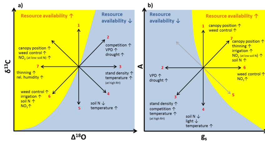
Figure 1 : The updated dual C-O isotope model according to Scheidegger et al., (2000). Arrows compare “two varying situations: A and B” as explained in the text. The symbol “ [?] ” indicates no significant change. Arrows pointing up (—) or down (—) stand for an increase/decrease of the respective values. \Delta^{18}\text{O} is the isotopic fractionation for ^{18}\text{O} vs. ^{16}\text{O} ; \delta^{13}\text{C} is the value for the stable carbon isotope; c_i/c_a is the ratio between the intercellular vs. ambient \text{CO}_2 mole fractions; A_{\text{net}} is the net photosynthesis (sensu Larcher, 2003); and g_s the stomatal conductance. Red dotted arrows show intermediate A_{\text{net}} - g_s -responses not covered in the original model.
