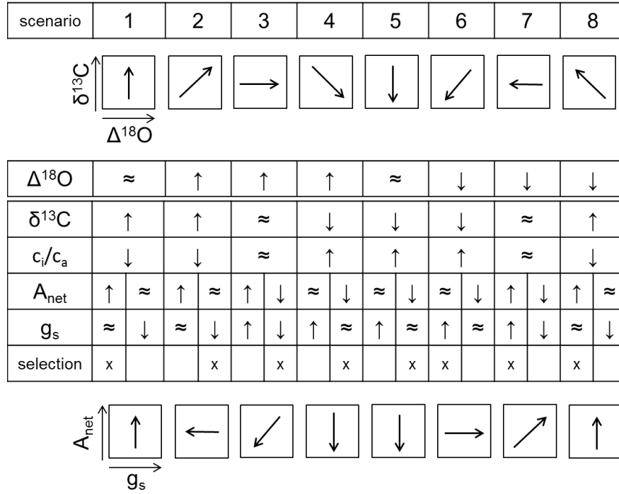
Figure 1 : The updated dual C-O isotope model according to Scheidegger et al., (2000). Arrows compare “two varying situations: A and B” as explained in the text. The symbol “ [?] ” indicates no significant change. Arrows pointing up (—) or down (—) stand for an increase/decrease of the respective values. \Delta^{18}\text{O} is the isotopic fractionation for ^{18}\text{O} vs. ^{16}\text{O} ; \delta^{13}\text{C} is the value for the stable carbon isotope; c_i/c_a is the ratio between the intercellular vs. ambient \text{CO}_2 mole fractions; A_{\text{net}} is the net photosynthesis (sensu Larcher, 2003); and g_s the stomatal conductance. Red dotted arrows show intermediate A_{\text{net}} - g_s -responses not covered in the original model.
