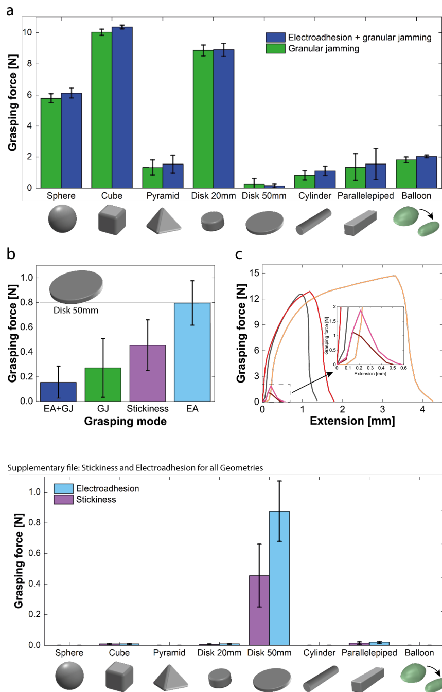
S1. Stickiness and electroadhesion for all geometries. The grasping forces in electroadhesion mode and using the nature stickiness of silicone are significantly higher in the case of a flat object, which fully covers the active area of the gripper.
