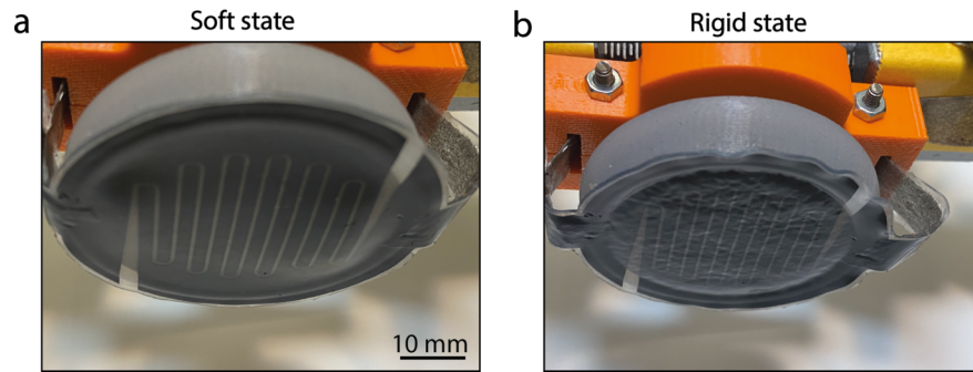
S2. Surface of the gripper's active area. a) In the soft state, the gripper's surface is smooth. b) After the activation of GJ triggered by air evacuation, all the granules stuck together causing the asperities formation on the surface of the gripper in the rigid state.
