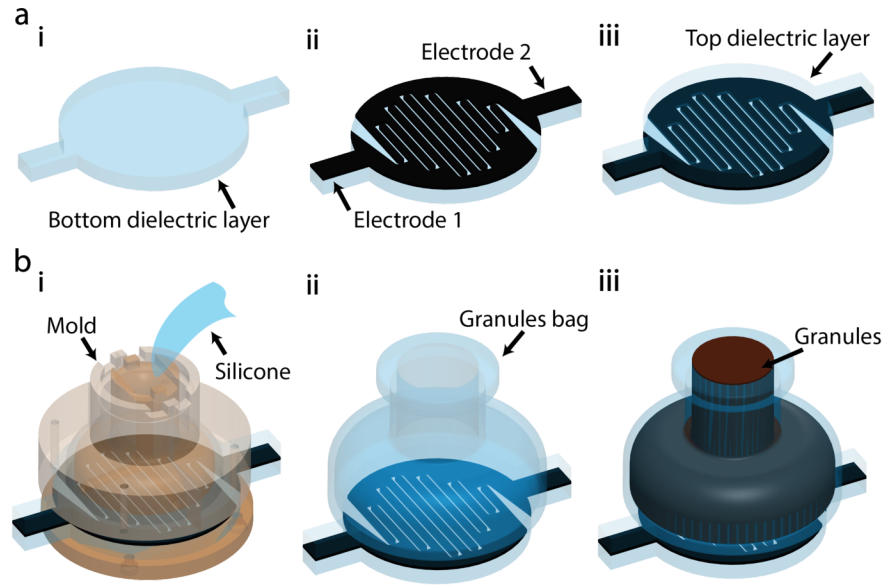
Figure 3. Fabrication process of the gripper. a) Electrode pad fabrication. A three-layer structure, which consists of a bottom silicone layer (i), a conductive silicone layer (ii), and a top silicone layer (iii) is blade-casted and cured in an oven one on top of the other. The electrode pattern (ii) is engraved using CO 2 ablation before the top silicone layer (iii) is cast. b) i) The fabricated pad is placed in an empty mold. Then, liquid silicone is poured into the mold to form the silicone bag and simultaneously connect the bag and the pad in a monolithic structure. ii) The silicone is solidified by thermal curing and the gripper is removed from the mold. iii) The silicone bag is filled with coffee granules (in brown).
