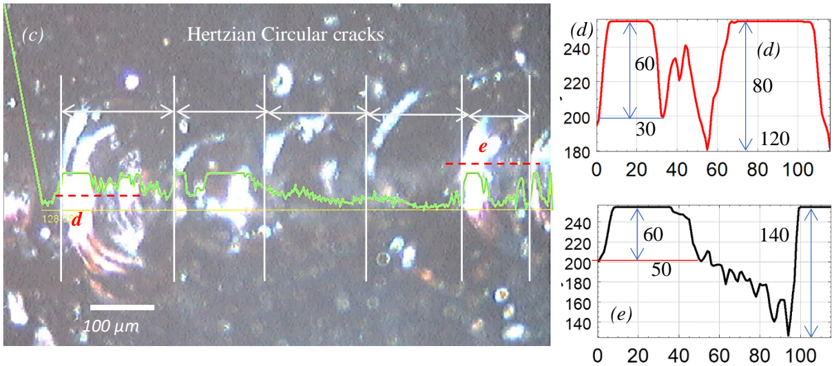
Fig 5. Scratch test with 10N/mm loading rate for Si Substrates showing plots of (a) Normal load and Tractional force vs. stroke length, (b) C.O.F vs. normal load and (c) the optical micrograph of the scratch track showing failure by circular cracking and surface intensity profile. The films were deposited at 100 °C in RF mode . Linear profiles of the regions marked (d) for higher loads (e) lower loads [21]
