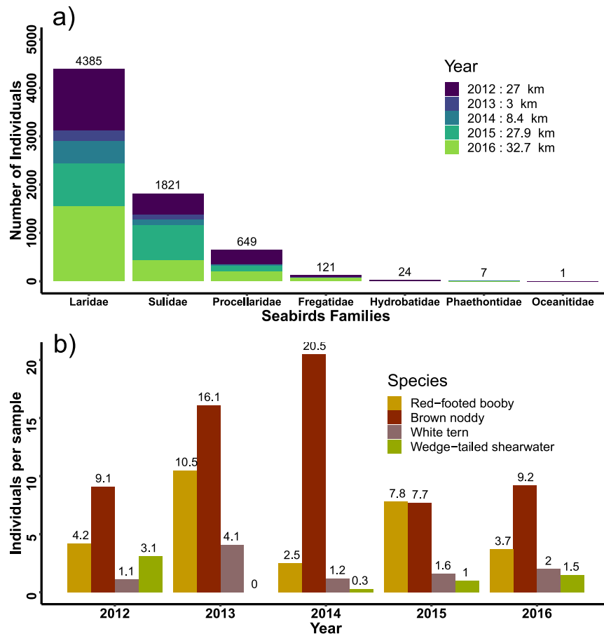
Figure 3: Number of individual seabirds by family summed across year (a) and for the four most abundant species red-footed booby ( Sula sula ), brown noddy ( Anous stolidus ), white tern ( Gygis alba ) and wedge-tailed shearwater ( Ardenna pacifica ) standardised by the number of samples for each year (b).
