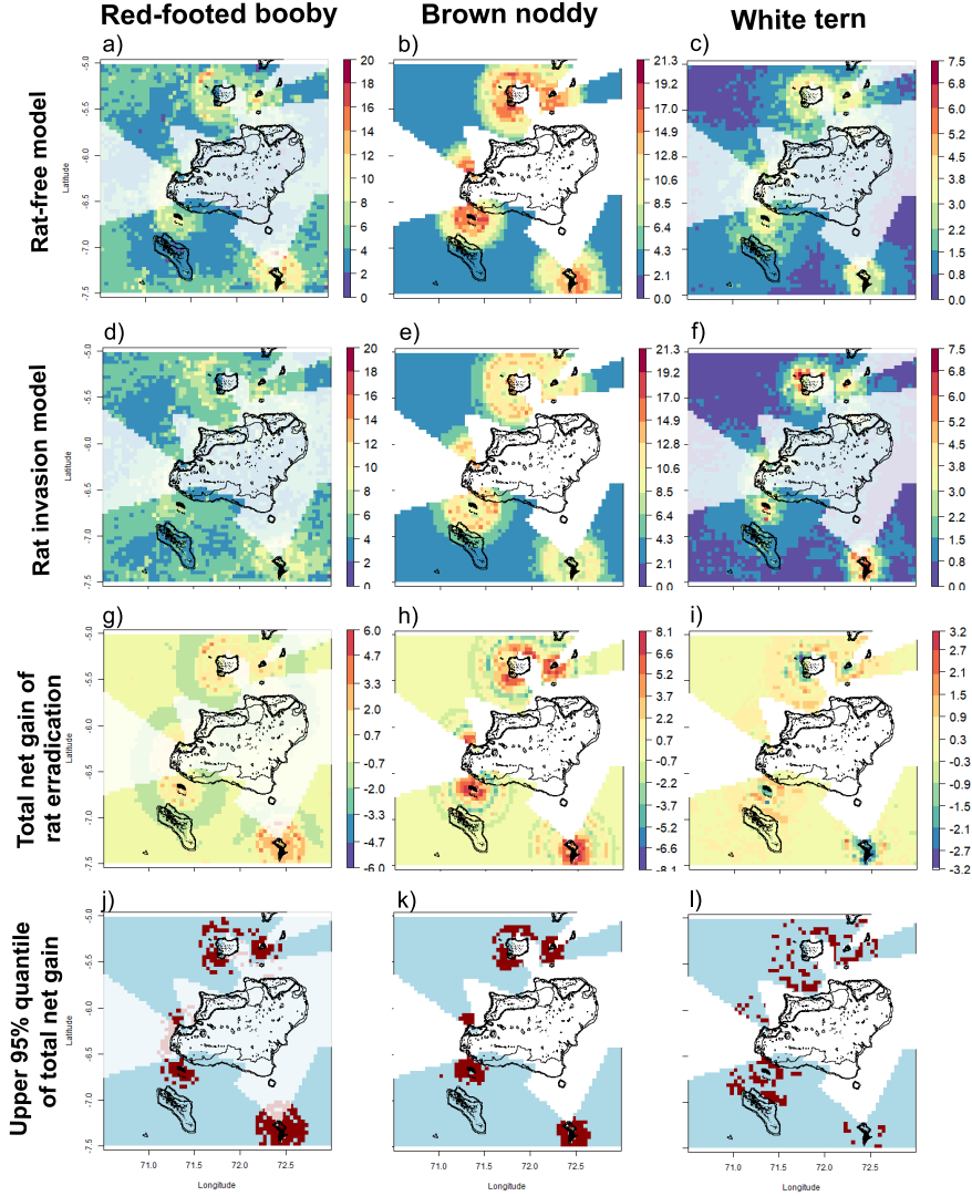
Figure 9: Predicted areas of increase in seabird abundance under a scenario of rat-eradication. Rat-free distribution predicted from BRT model using a rat-free scenario (a-c), and a rat-invaded scenario (d-f), where each island is set as either ‘rat-free’ or ‘rat-invaded’ respectively. These models represent the distribution predictions under complete eradications of rats and a full invasion of rats respectively. Hence, an approach to understand the variations of distribution is calculated by subtracting the rat-invaded minus the rat-free models. This yielded to the net gain in bird abundance under a scenario of rat eradication (g-i). The upper 95% quantile increase of the net gain is also showed (j-l). White shaded areas indicate areas nearby currently rat-free islands in which a rat eradication programme would not have any effect since they are already at the theorised maximum abundance.
