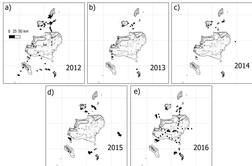
Figure 2: Year-to-year sampling effort in the Chagos Archipelago. Each 300 m transect is represented by a black dot as the spatial resolution does not allowed us to perfectly draw lines.
