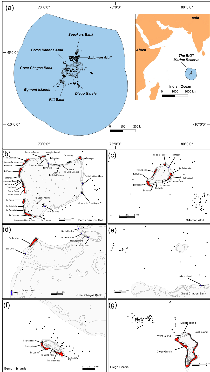
Figure 1: Seabird sampling effort within the Chagos Archipelago and the British Indian Ocean Territory. Boundaries of the BIOT MPA (a), and locations within the Indian Ocean (inset). Individual atolls and islands (b-g). Black dots represent the location of individual bird transects. Rat-invaded islands are coloured in red and rat-free islands in blue. Six islands have been reported with uncertain rat status (Île Verte, Île Manon, Île Finon, Île de la Passe and a small Unnamed Island in Peros Banhos) and are for representation purposes shown as rat-invaded.
