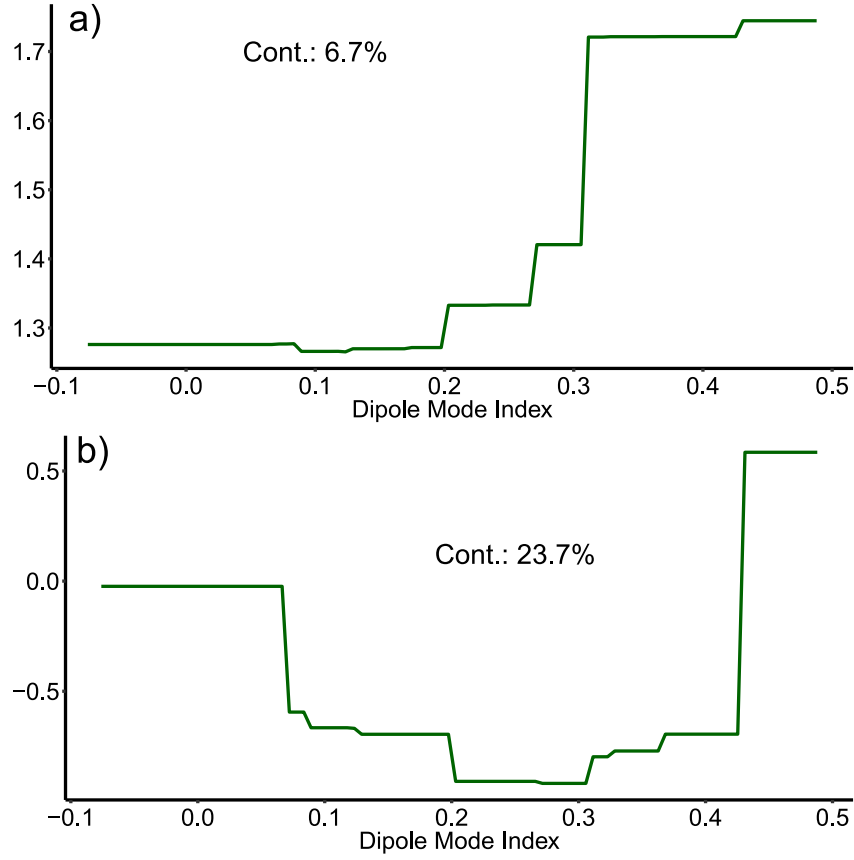
Figure 5: Partial dependence plots of the response of red-footed booby (a) and wedge-tailed shearwater (b) to Dipole Mode Index. Both species show a positive correlation with increasing positive DMI. Positive DMI means cooler temperature in eastern Indian Ocean and warmer temperature in western Indian Ocean.
