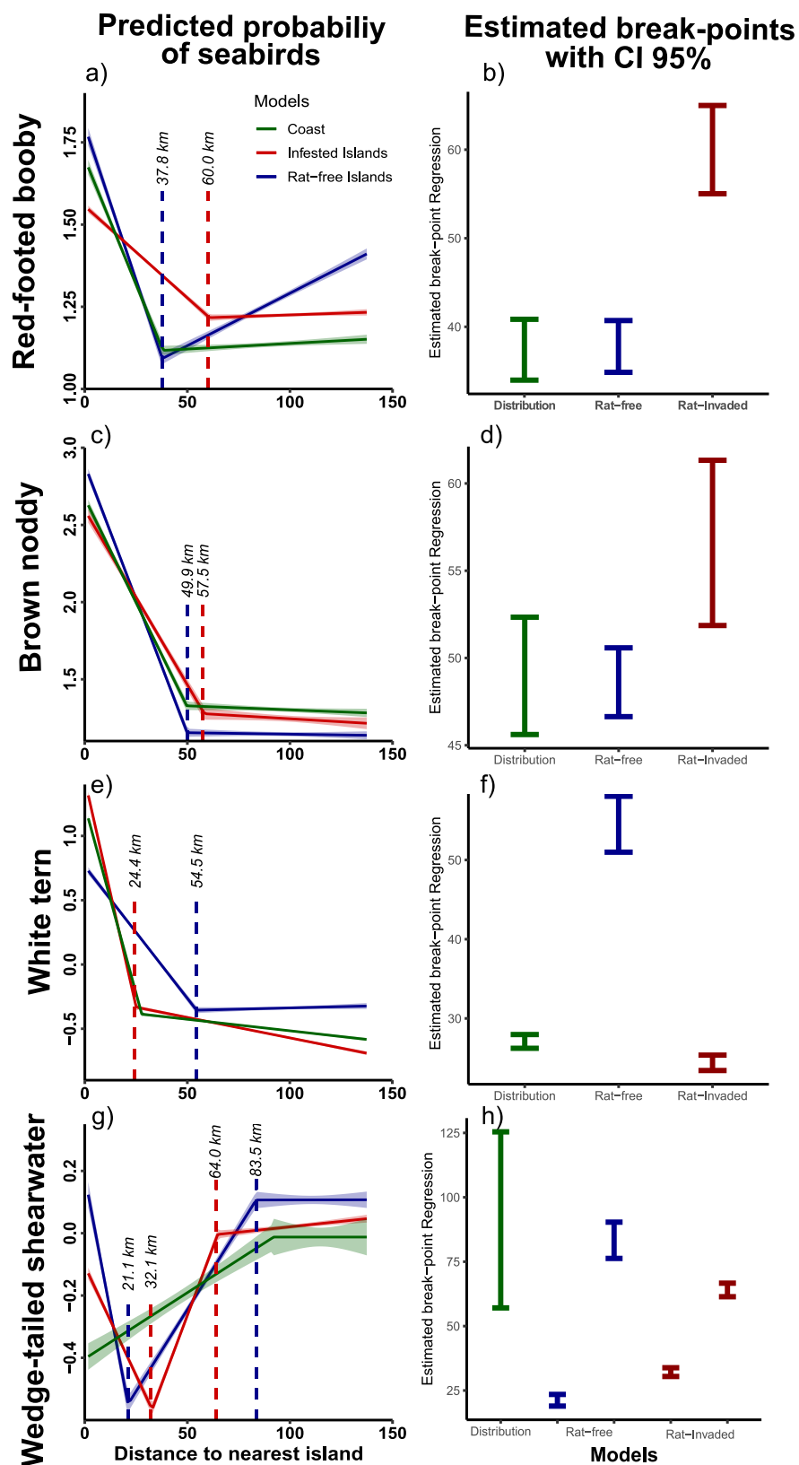
Figure 8: Sensitivity of seabird distribution to presence or absence of rats on nearby islands. Partial dependence plot (a, c, e, g) of the effects of rat-free (blue lines) and rat-invaded (red lines) islands contrasted with the original distribution model (green lines). Stippled line denotes location of the breaking point that denotes a threshold in distribution. Comparison of the break point regression using the 95% confident intervals calculated in the Davies' test is shown (b, d, f, h)
