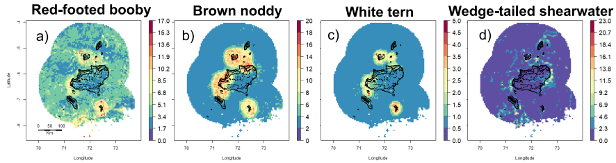
Figure 6: Predicted distribution of red-footed booby, brown noddy, white tern and wedge –tailed shearwater as a function the BRT models. Colour scales represent the seabird abundance response, ranging from highest predicted value (red) to zero (blue). Scales differ between species as a function of difference in abundance. Predictions were run within the convex hull of the variables.
