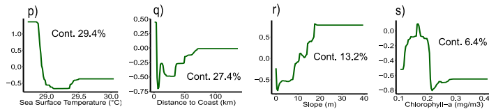
Figure 4: Partial dependence plots of each variable modelled in the BRTs for all four species. The green-solid line in each graph represents the response of the species to the variables. The relative contribution of the model is showed from the greatest to the least. Plots manifest that non-monotonic responses were found.
